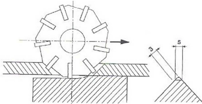
VCF-700 Side mill cutter
